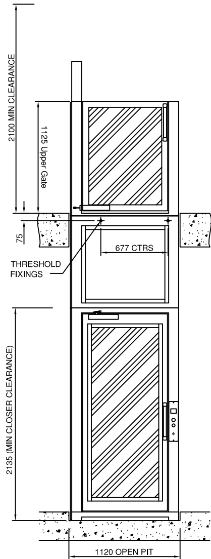
FRONT ELEVATION
