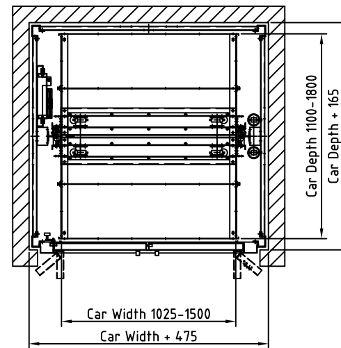
View C View A View B Shaft Plan
