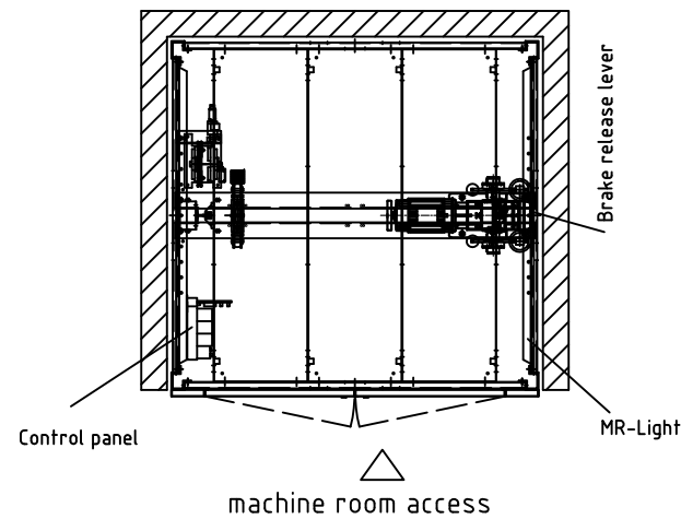
Machine Room Plan
