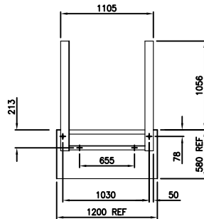
HOLES DRILLED BY INSTALLATION ENGINEERS GATE FRAME FIXINGS
