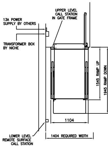
PART PLAN VIEW
