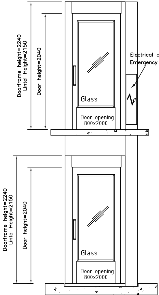
View A
